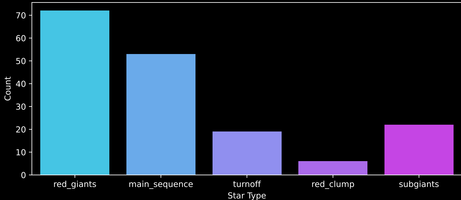
APOGEE DR17 Field: [N188-RV] Count plot of Star Type
