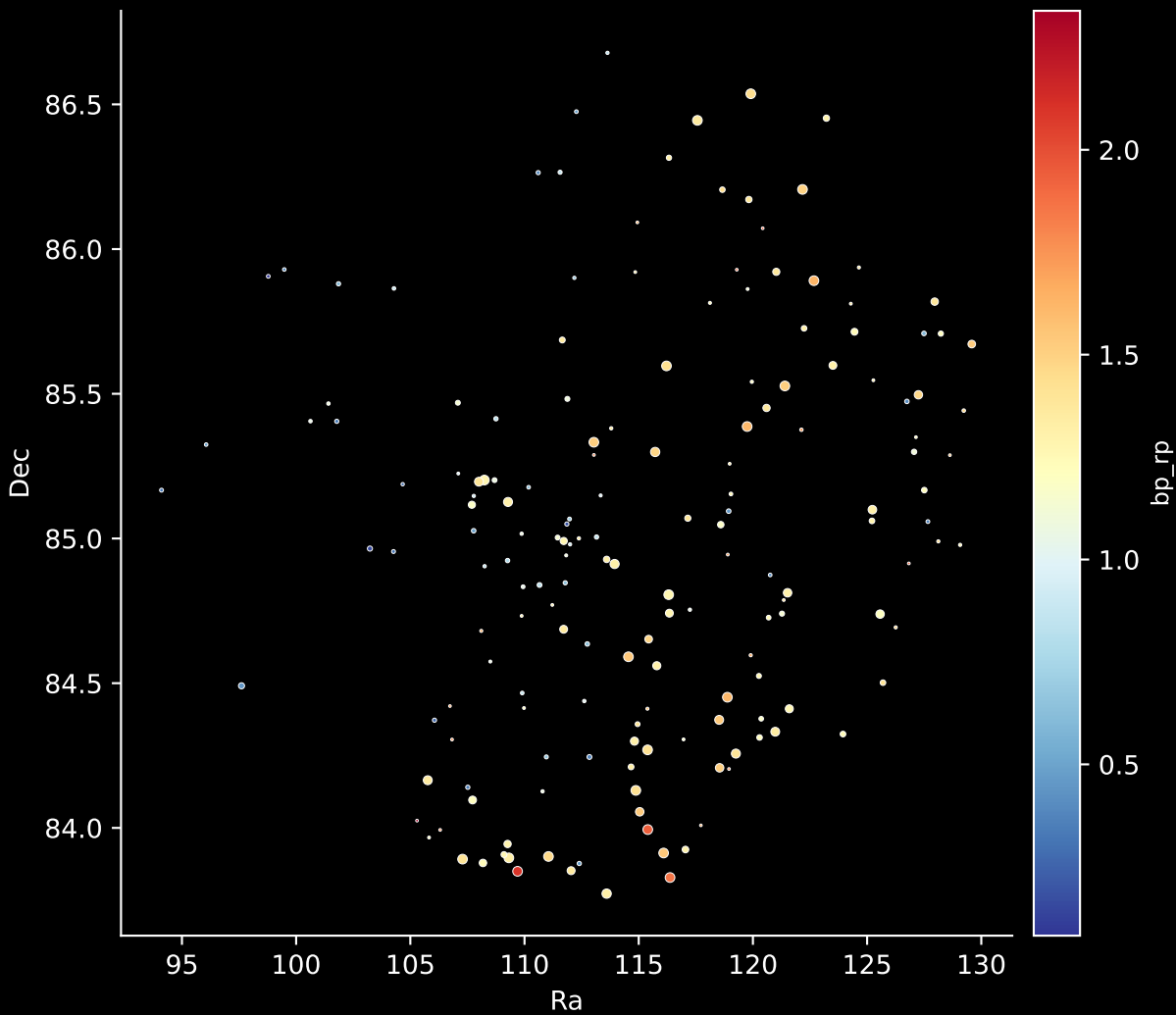
APOGEE DR17 Field: [N188-RV] Stars: 172
