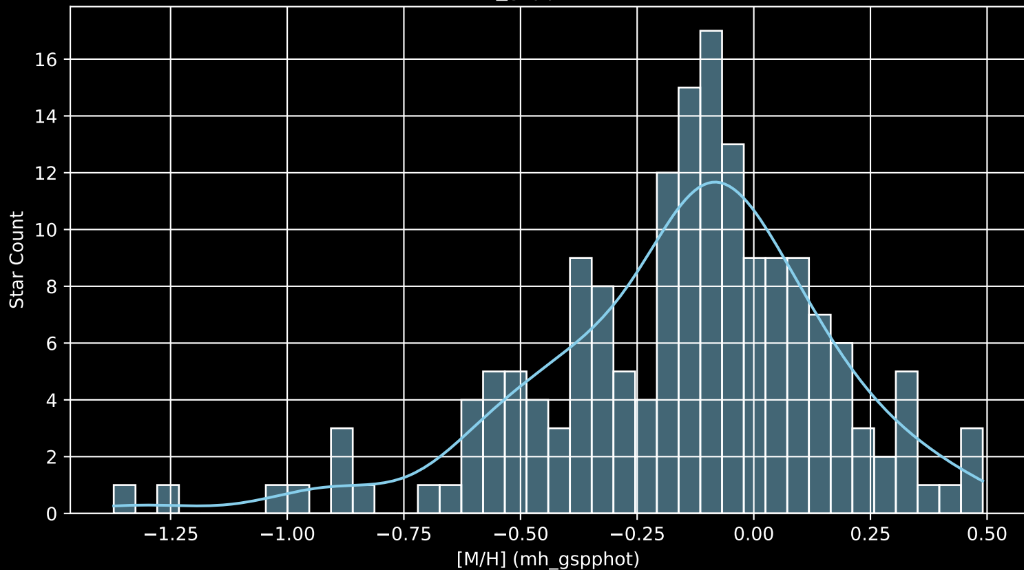
APOGEE DR17 Field: [N188-RV [M/H] (mh_gspphot) (n= 169)
