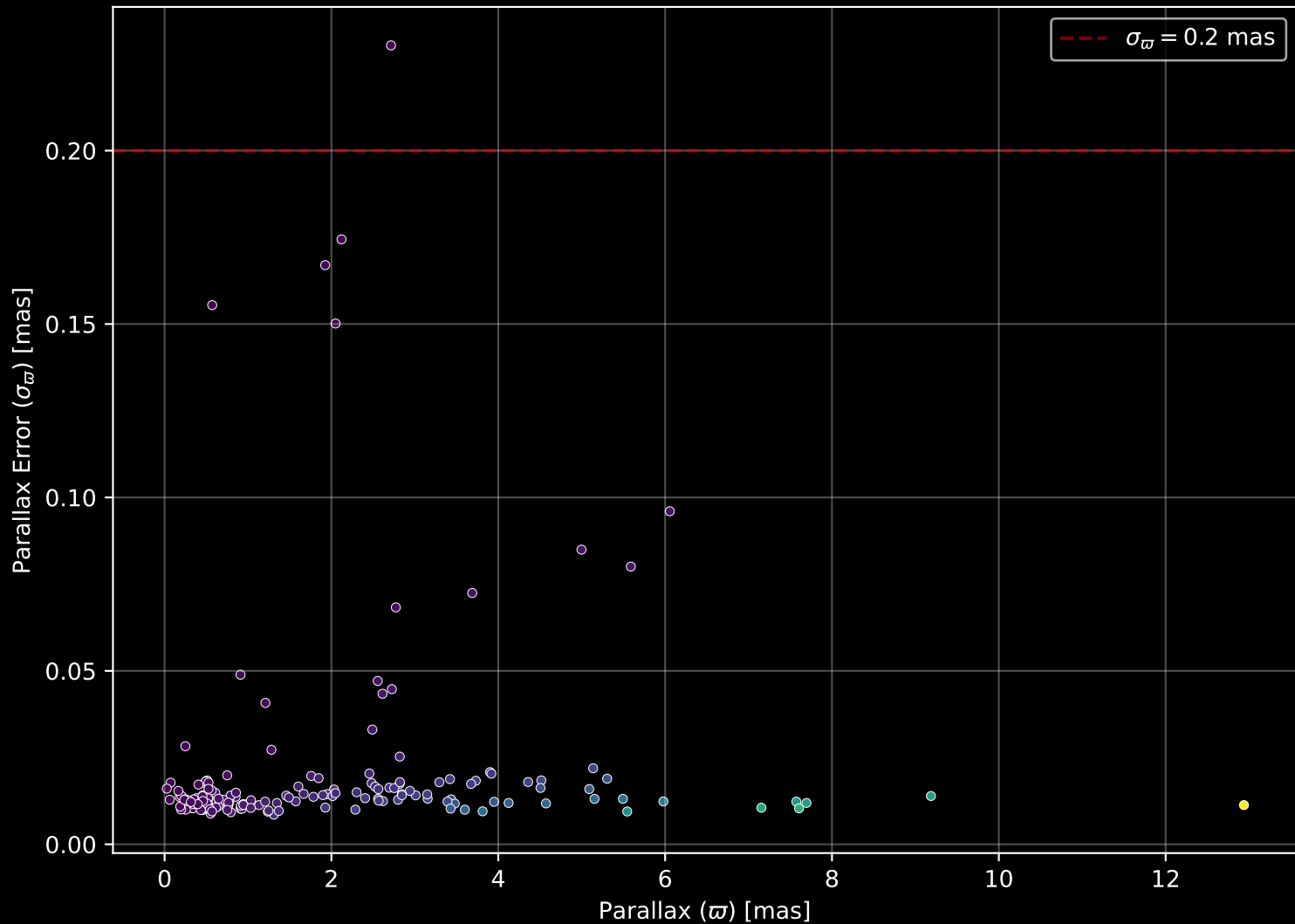
APOGEE DR17 Field: [N188-RV] Parallax Quality (n= 172)
