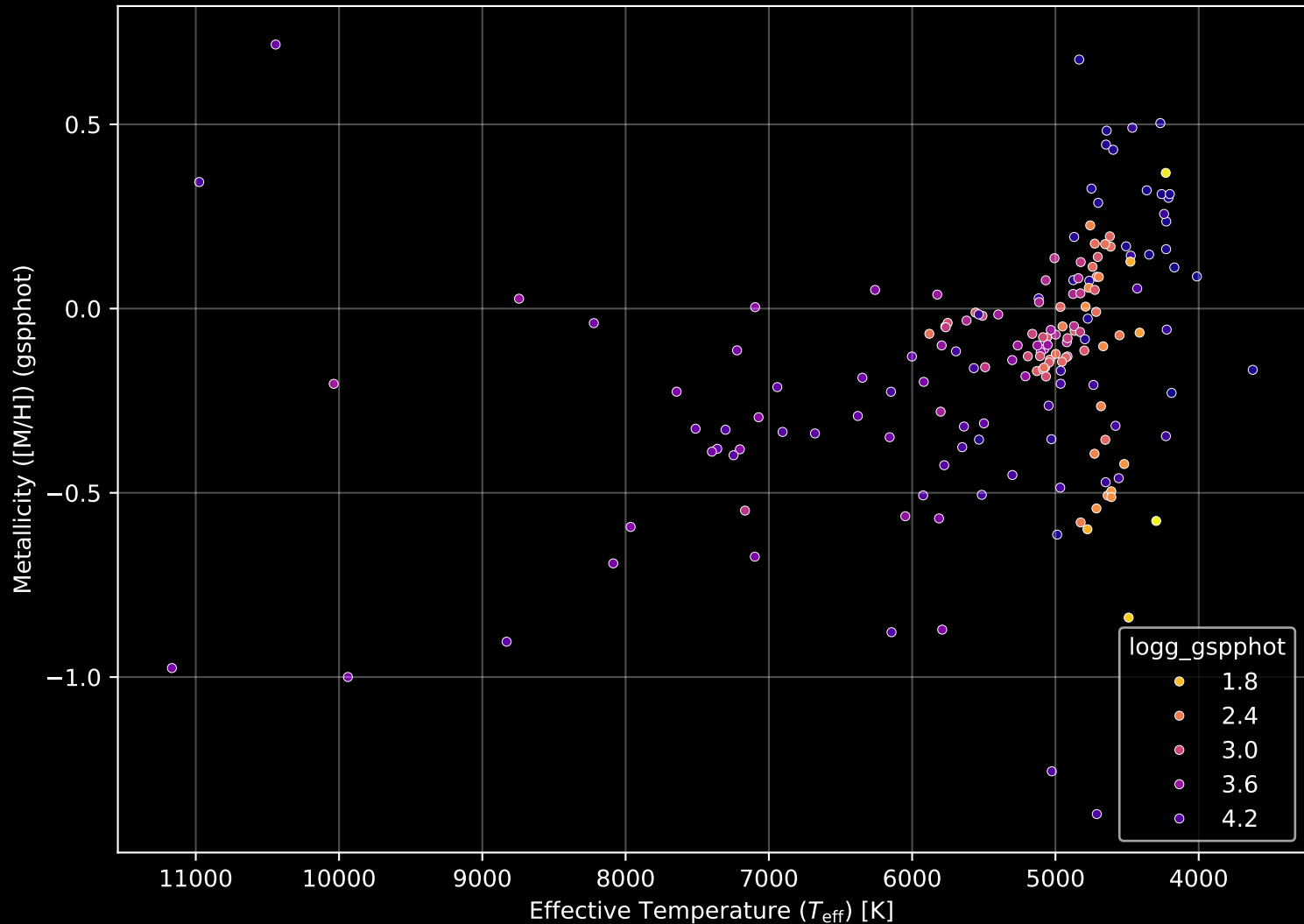
APOGEE DR17 Field: [N188-RV] Stellar Population Parameters (n= 172)
