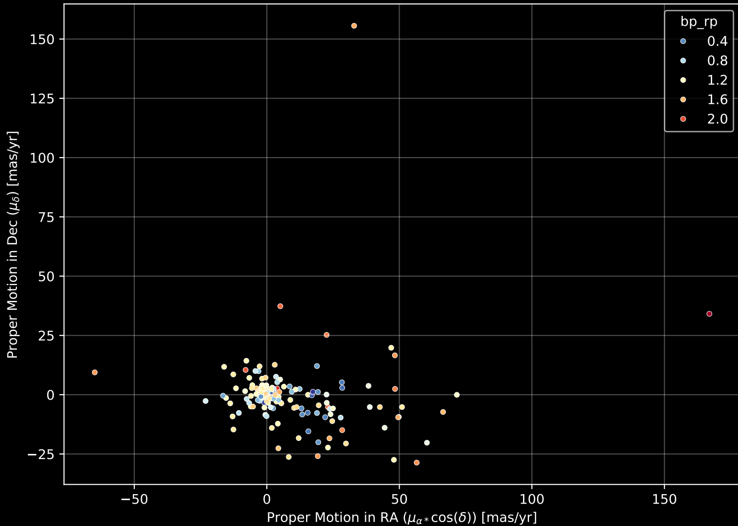
APOGEE DR17 Field: [N188-RV] Proper Motion Diagram (n= 172)
