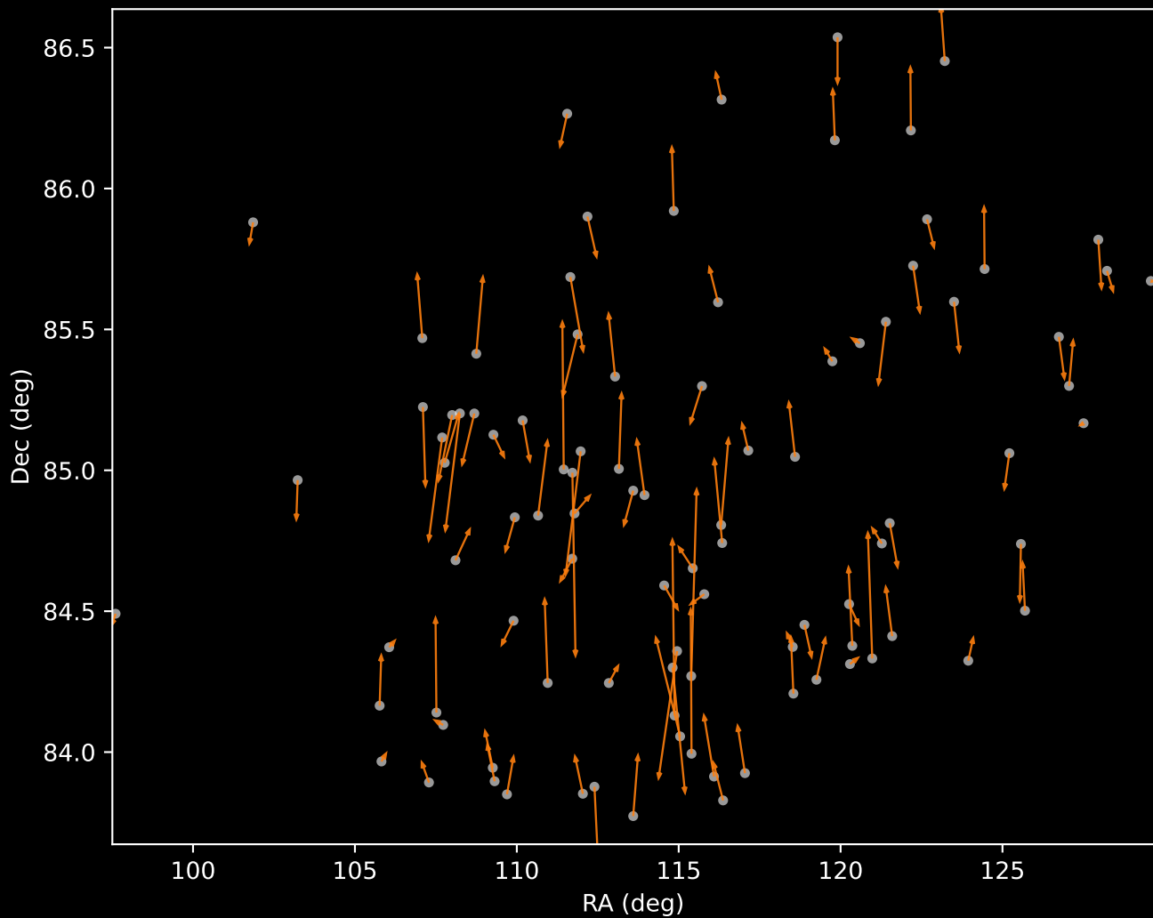
APOGEE DR17 Cluster 2 Proper Motion Vectors (n=96)
