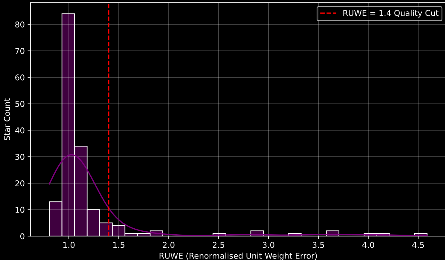
GAPOGEE DR17 Field [N188-RV] RUWE Distribution (n= 163)
