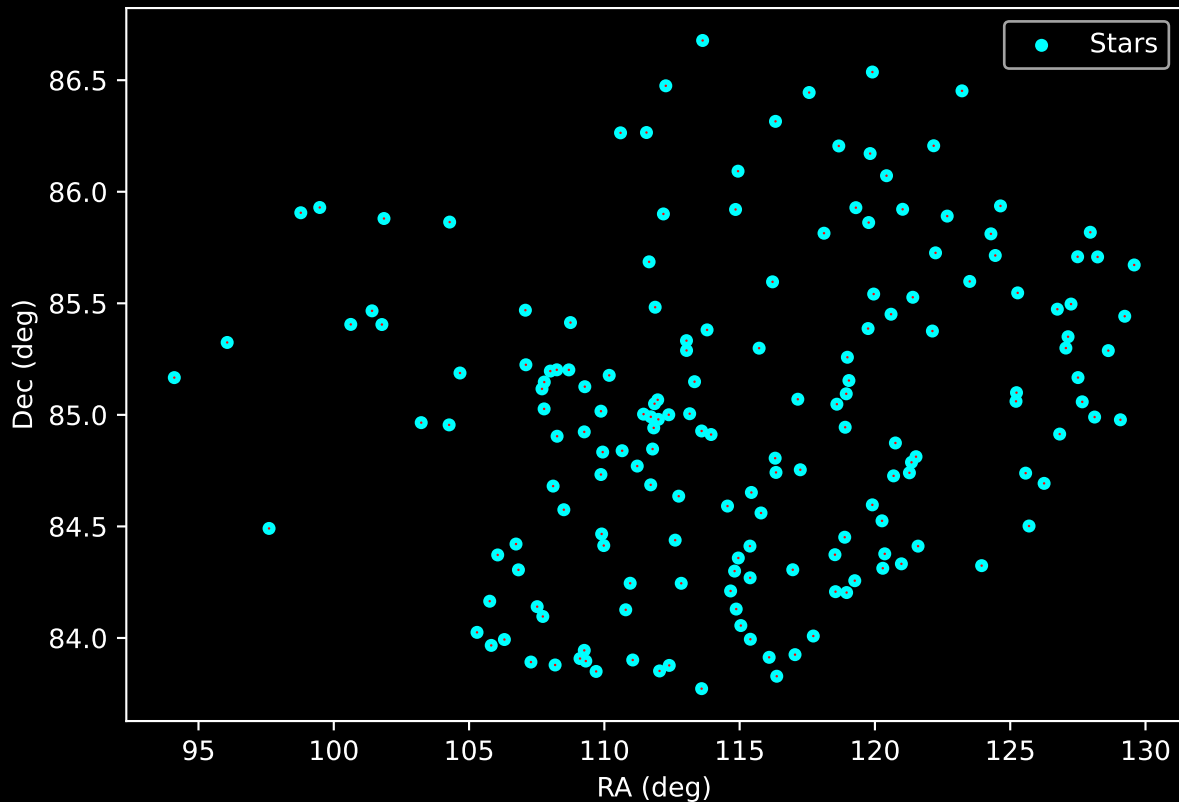
APOGEE DR17 Field: [N188-RV] Proper Motion Vectors for Gaia Star Field (n= 172)
